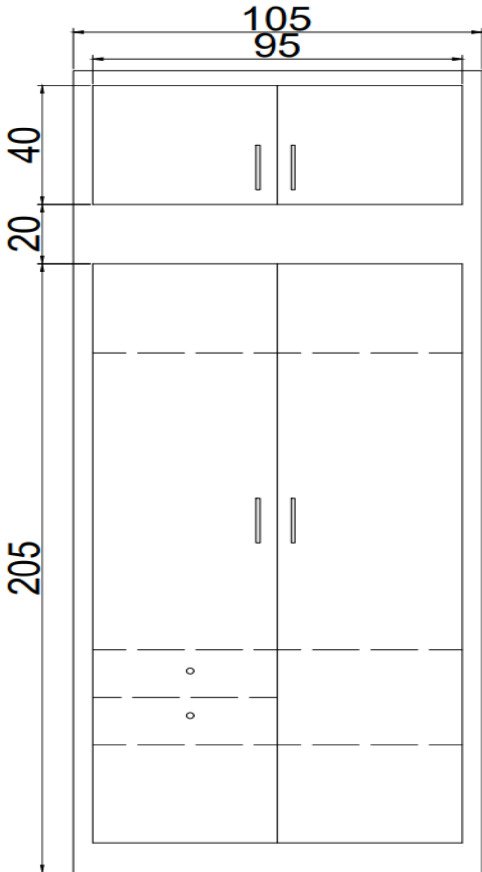
WARDROBE DETAILS
