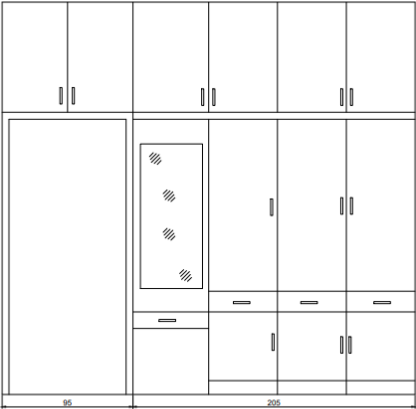
WARDROBE - 2 - VIEW WITH SHUTTERS
