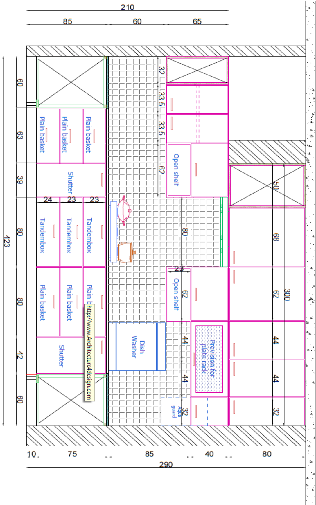
ELEVATION C
