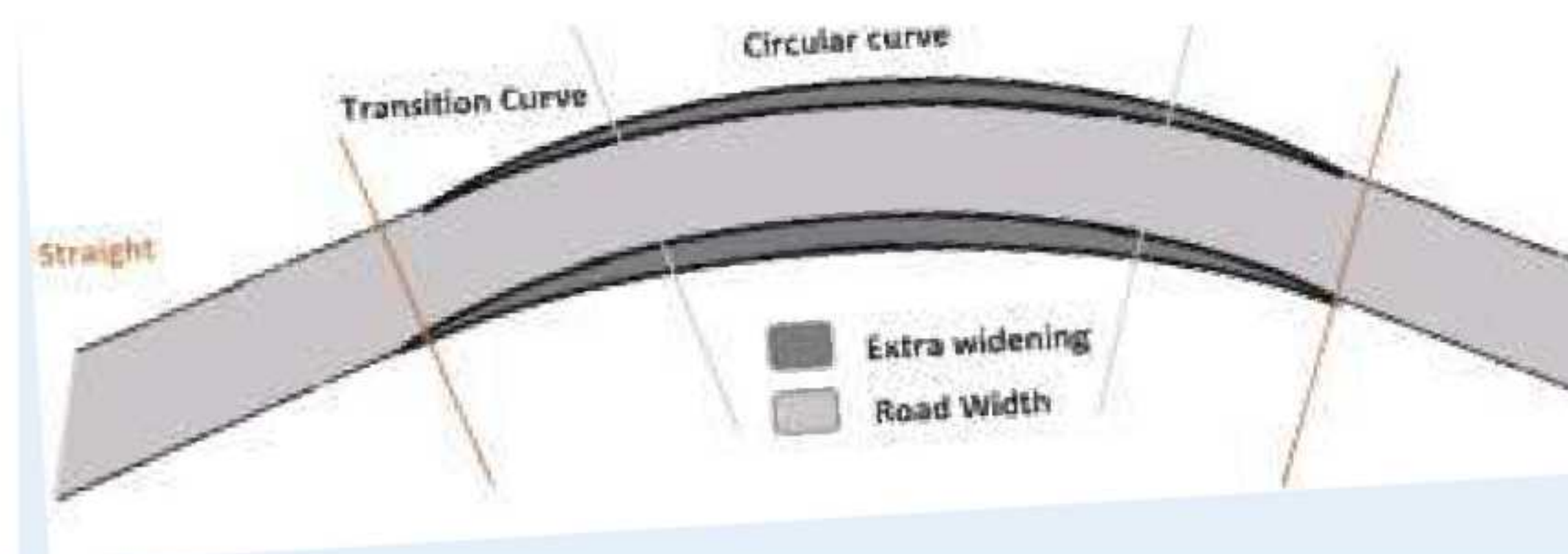
Figure 3.1: Extra widening on road curve
