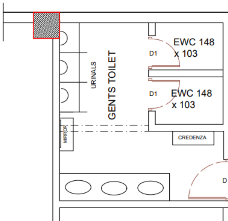
LAYOUT OF PROPOSED GENT'S WASHROOM AT FIRST FLOOR
