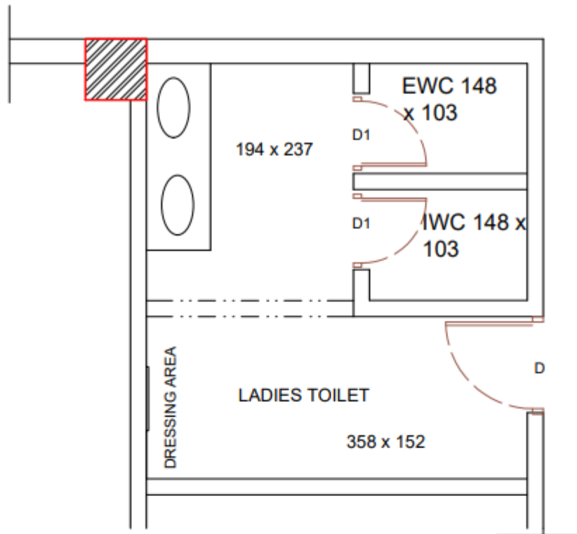
MAIN OFFICE - LAYOUT OF EXISTING LADIES WASHROOMS AT FIRST FLOOR
