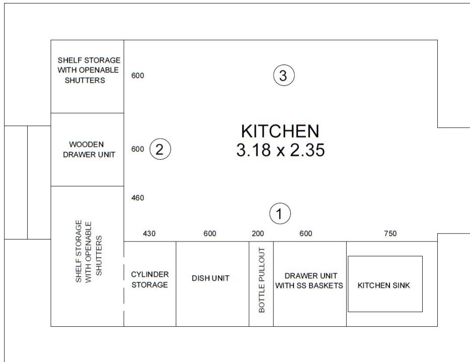
MODULAR KITCHEN TENTATIVE LAYOUT
